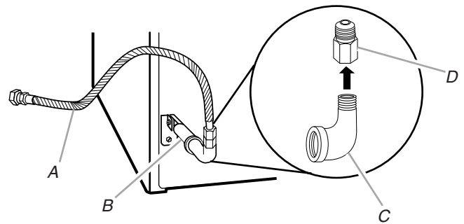
A. \frac{3}{8} " flexible gas connector B. \frac{3}{8} " dryer pipe C. \frac{3}{8} " to \frac{1}{2} " pipe elbow D. \frac{1}{2} " pipe-to-flare adapter fitting
